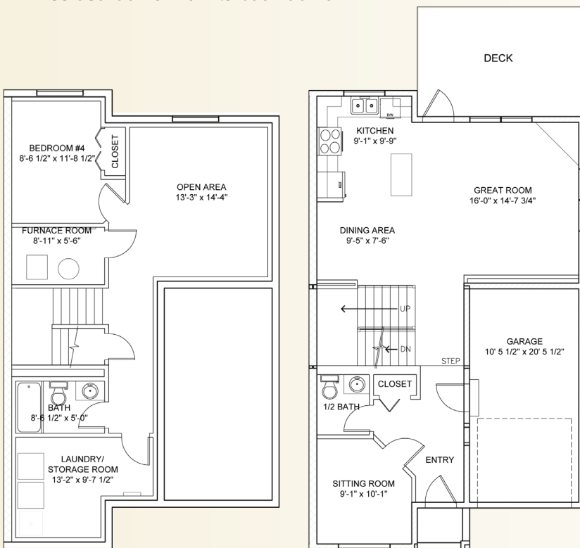
Basement - 810 sq. ft.
