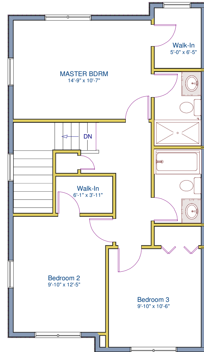
Upper Floor 745 sq. ft
